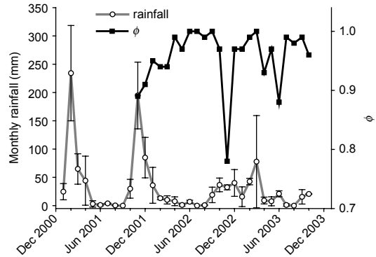
Fig. 4. Monthly rainfall (mm) and Keeling's clustering coefficient \phi of the association data during the course of the study. Mean and standard deviations of the monthly rainfall were calculated using four rainfall stations in the Satara region of the Kruger National Park. Rainfall data from 2000 to 2001 are shown to contrast the below-average wet season in 2002–2003.
